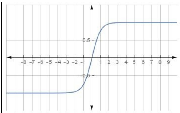
Hyperbolic tangent
