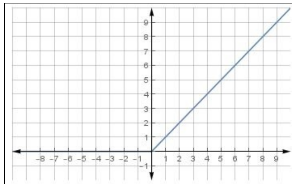
ReLU
